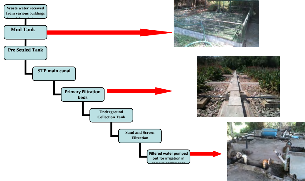
Operational Diagram of Sewage Treatment Plan (STP)
